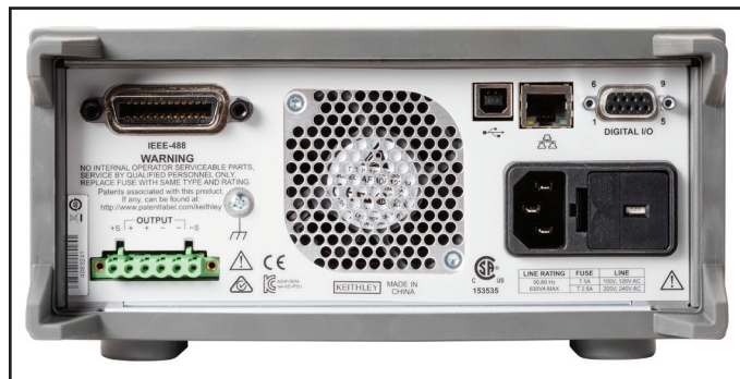
Figure 7. 2281S rear panel.
